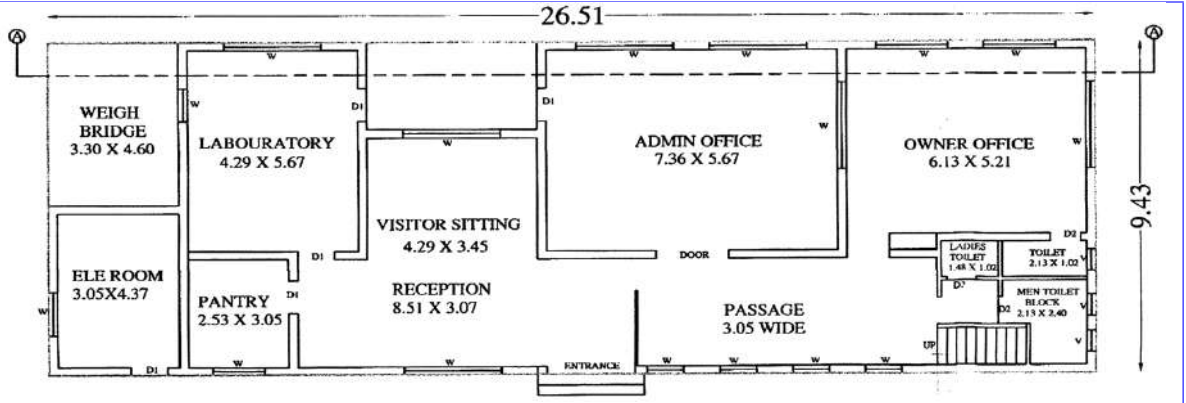
Ground Floor Plan cum Site Plan
